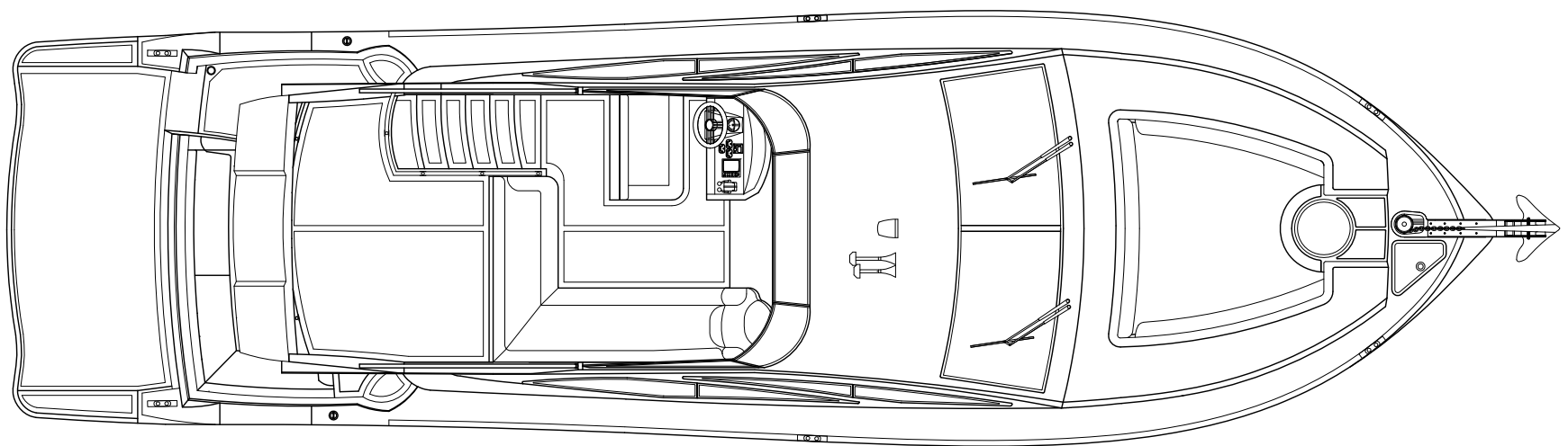
SUN DECK PLAN
