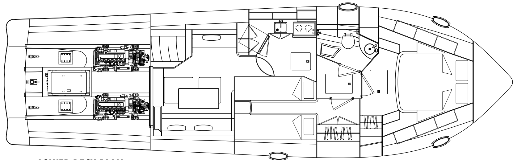
LOWER DECK PLAN
