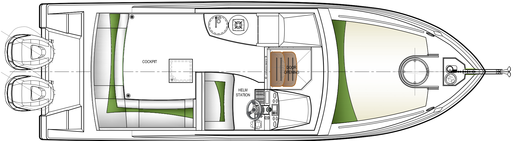
DECK PLAN
