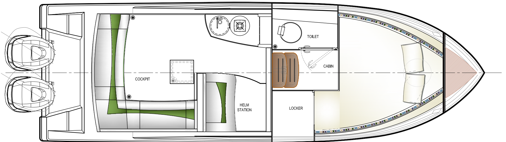
GENERAL ARRANGEMENT PLAN
